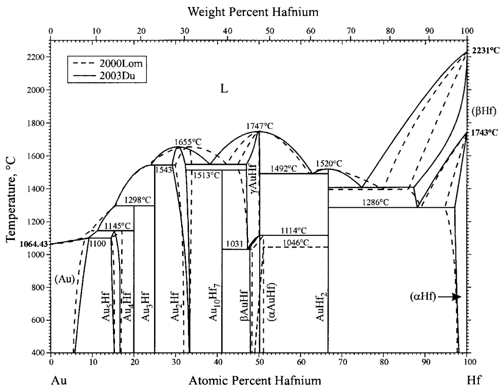
Fig. 1 Au-Hf phase diagram
